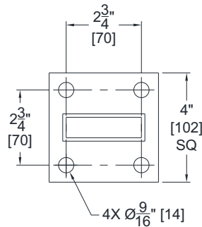
BASE DETAIL
