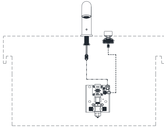
3801-H-MXTP DIAGRAM (SHOWN FOR REFERENCE)
